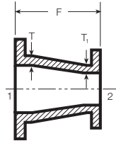
Concentric Reducer
