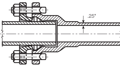
A-702 2" Mechanical Joint Pipe A-802 2 1/4"
