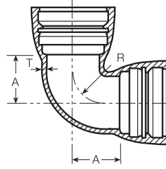
Lok-Ring Bell-Bell**
