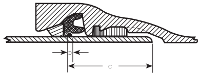
Flex-Ring® Joint 14"-60"
