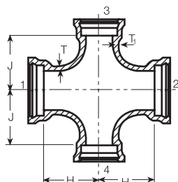
A-21 All Bell
