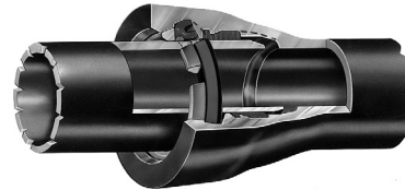
14"-60" Flex-Ring® Joint
