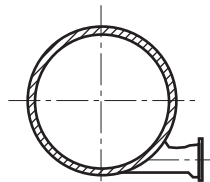
Blow-Off Branch
