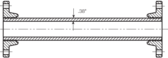
A-706 2" Flange and Flange Pipe
