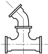
MJ Tee with MJ & PE 45° Bend
