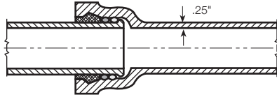
A-701 2" Bell and Spigot Pipe A-801 2 1/4"
