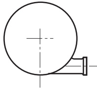
Tangential Welded-on Outlet (See Section 7)
