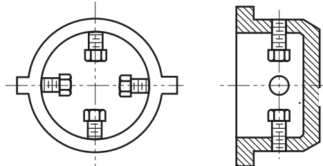
A-20803 Restrained Plug
