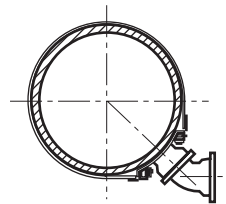
Saddle & 45° or 60° Bend (See Section 7)
