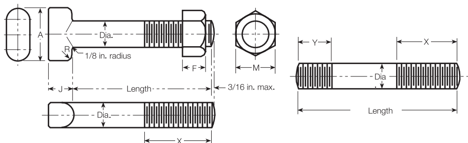
Tee Head Bolt
