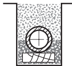
D - Pipe Laid on Blocks Tamped Backfill
