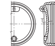
54"-64" Lok-Ring Caps
