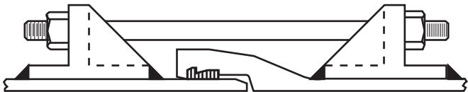
Lugged Fastite Joint
