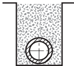
A - Flat Bottom Trench Untamped Backfill
