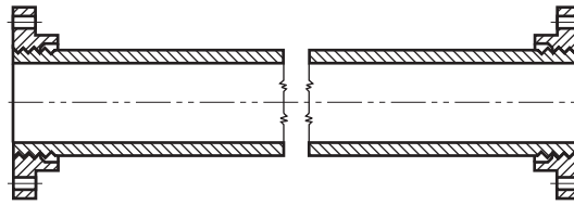
Flange and Flange
