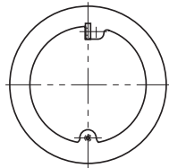
4"-48" Flex-Ring Caps
