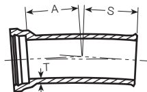
A-209 Bell & Spigot 5 5/8° Bend
