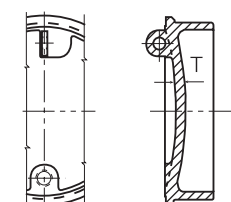
54"-64" Lok-Ring Plugs
