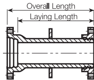
MJ-Thrust Collar-Flange
