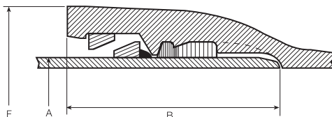
4"-12" Flex-Ring
