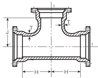
All MJ Tee
