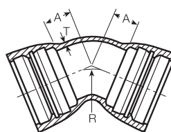
Lok-Ring Bell-Bell**
