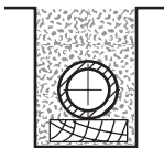
C - Pipe Laid on Blocks Untamped Backfill
