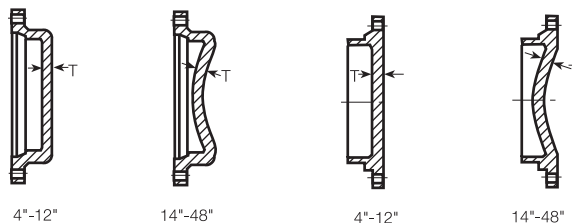
MJ Cap
